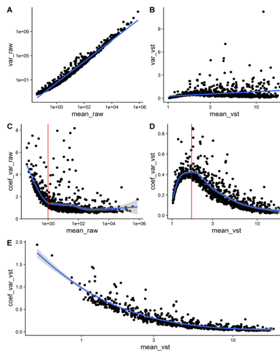
Supplementary Figure 2 Results of miRNAs quality control analysis on the log-log scale.
