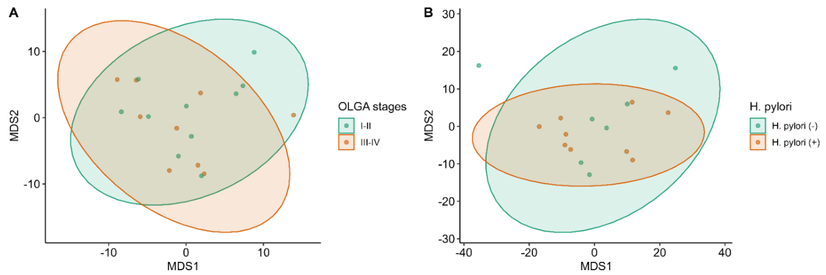
Supplementary Figure 3 Multidimensional scaling plots based on normalized data showing a clustering. A: corresponding to Operative Link on Gastritis Assessment staging of atrophic gastritis samples; B: corresponding to H. pylori infection status of gastric cancer samples. MDS: multidimensional scaling; OLGA: Operative Link on Gastritis Assessment; H. pylori (-): Helicobacter pylori -negative; H. pylori (+): Helicobacter pylori -positive.
