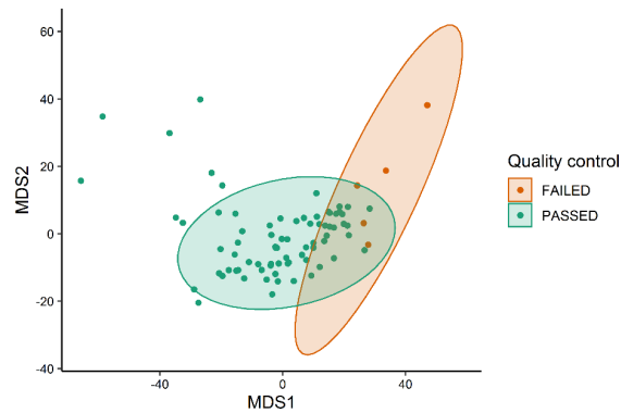
Supplementary Figure 1 Multidimensional scaling plot showing outliers of control, atrophic gastritis, and gastric cancer samples after quality control analysis. The analysis was performed based on sequencing depth ( > 1e6 of mapped reads) and the number of detected miRNAs ( > 1.5 interquartile range on \log_2 scale). MDS: multidimensional scaling.
