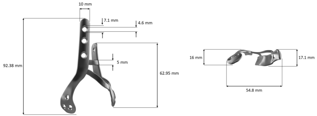
Supplementary Figure 2 Patient-specific plate.
