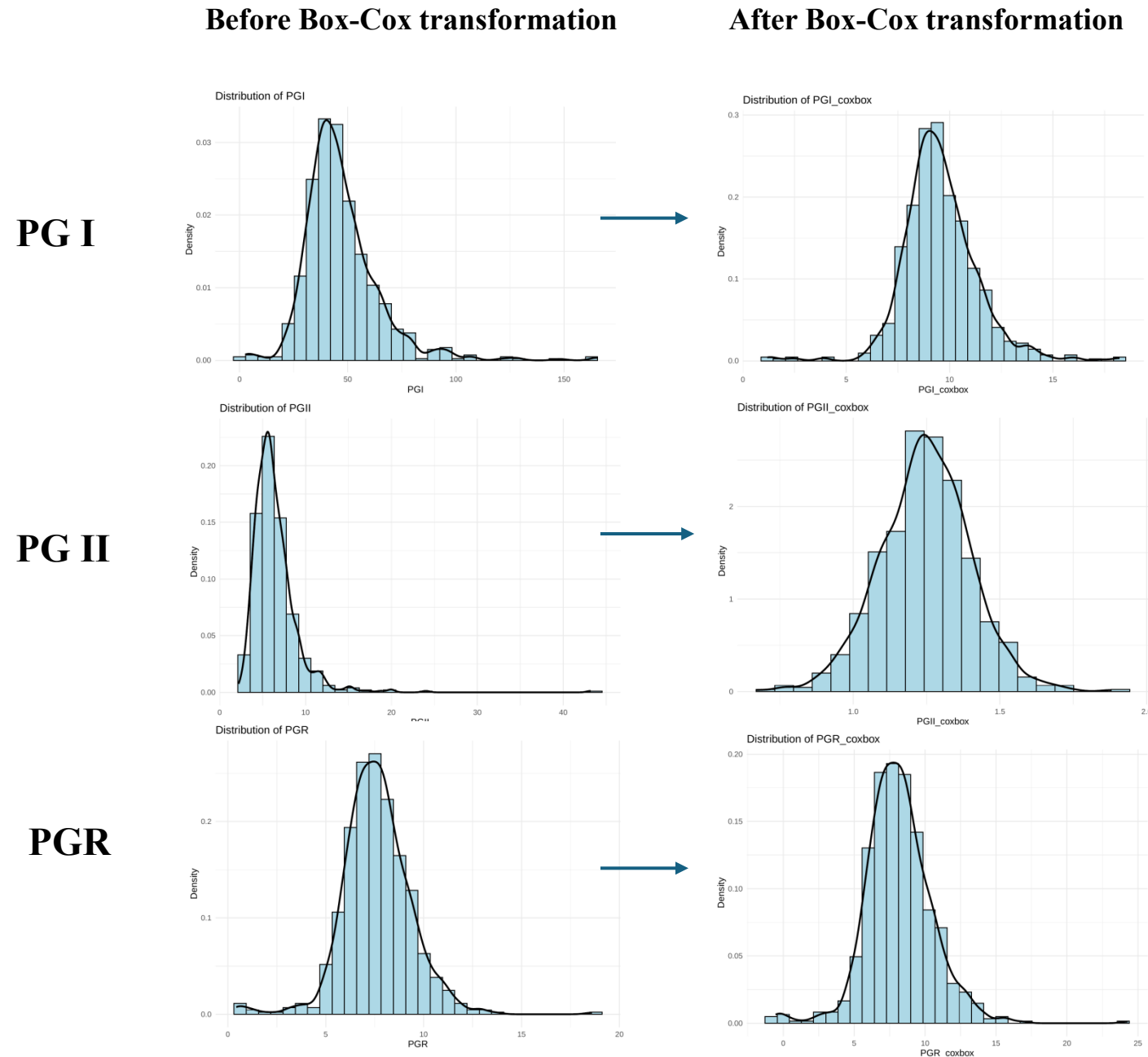
Supplementary Figure 1 Distribution of PG I, PG II, and PGR values before and after Box-Cox transformation. PG: Pepsinogen.
