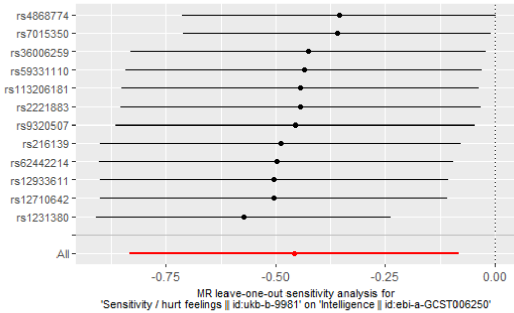
Supplementary Figure3 Leave-one-out plots for the analysis of sensitivity/hurt feelings on intelligence.
