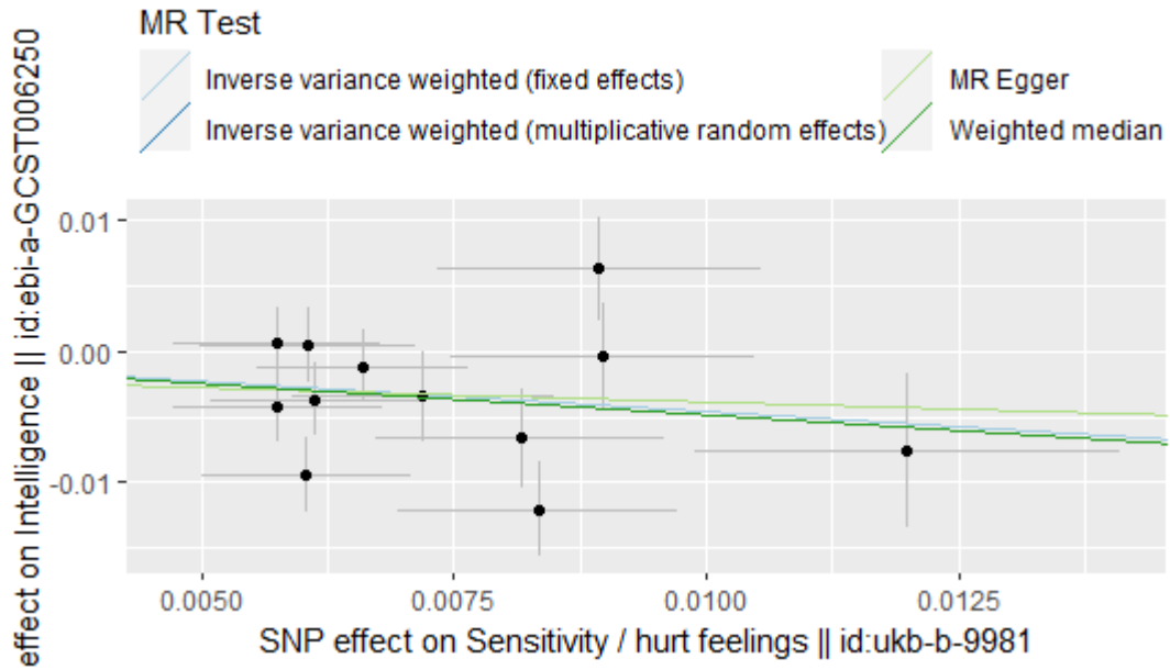
Supplementary Figure 1 Scatter plots for the analysis of sensitivity/hurt feelings on intelligence.
