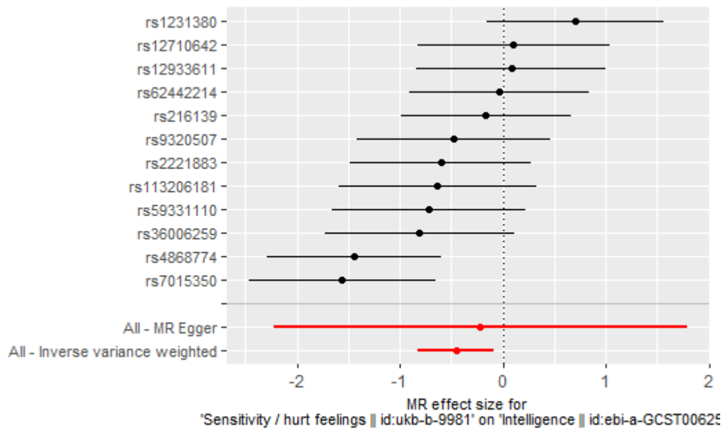
Supplementary Figure 2 Forest plots for the analysis of sensitivity/hurt feelings on intelligence.
