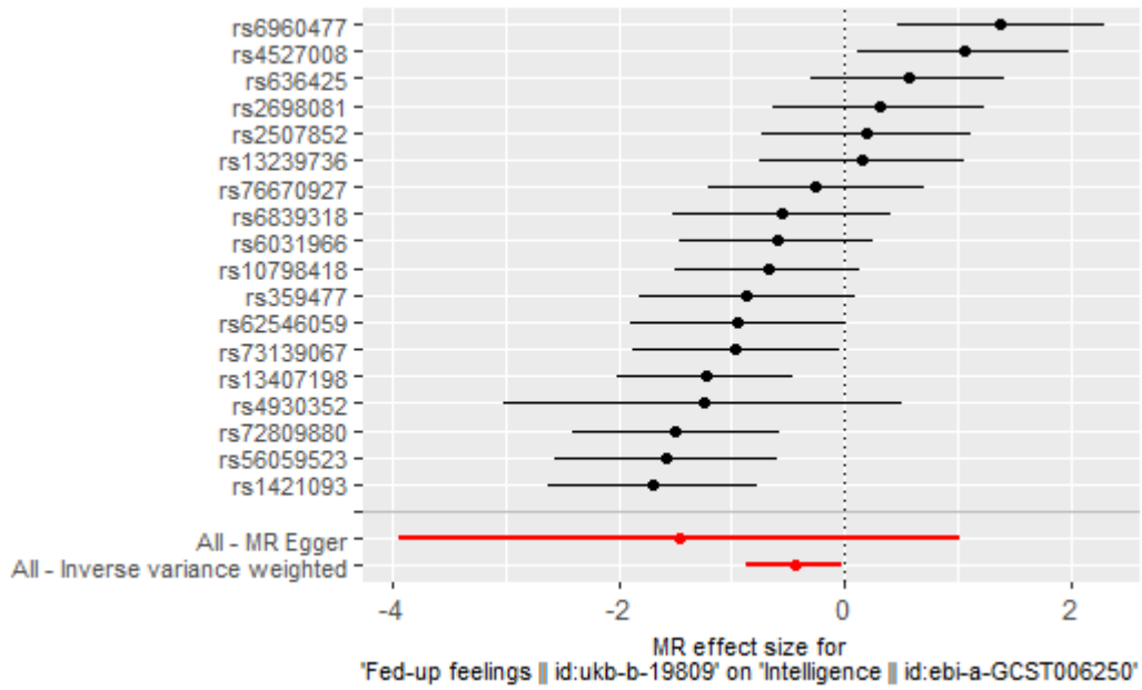
Supplementary Figure 5 Forest plots for the analysis of fed-up feelings on intelligence.
