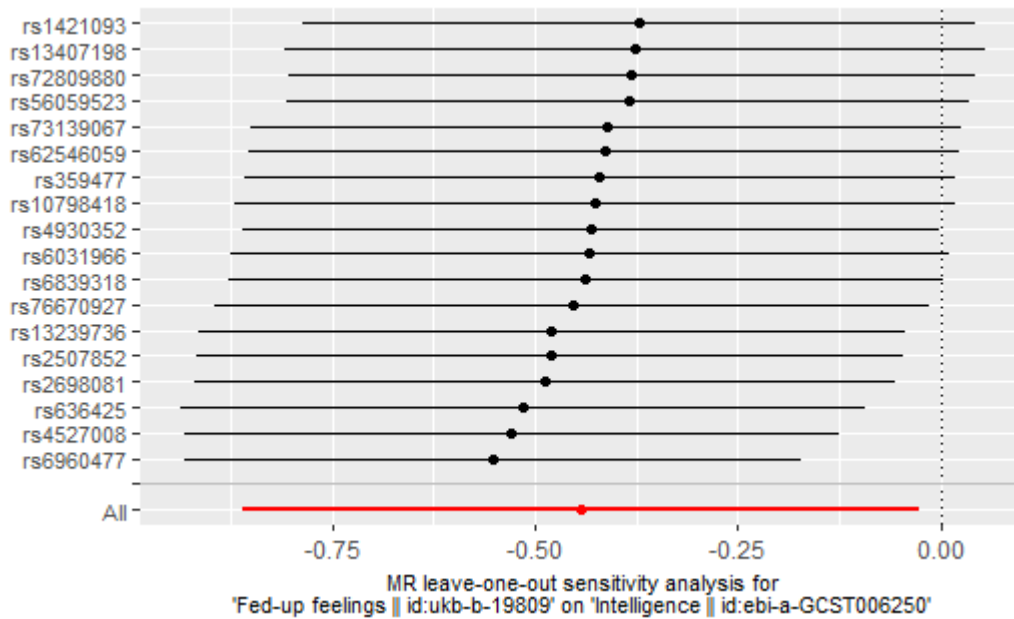
Supplementary Figure 6 Leave-one-out plots for the analysis of fed-up feelings on intelligence.
