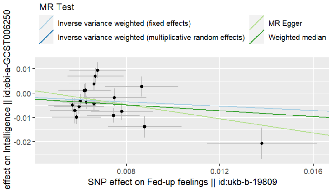
Supplementary Figure 4 Scatter plots for the analysis of fed-up feelings on intelligence.
