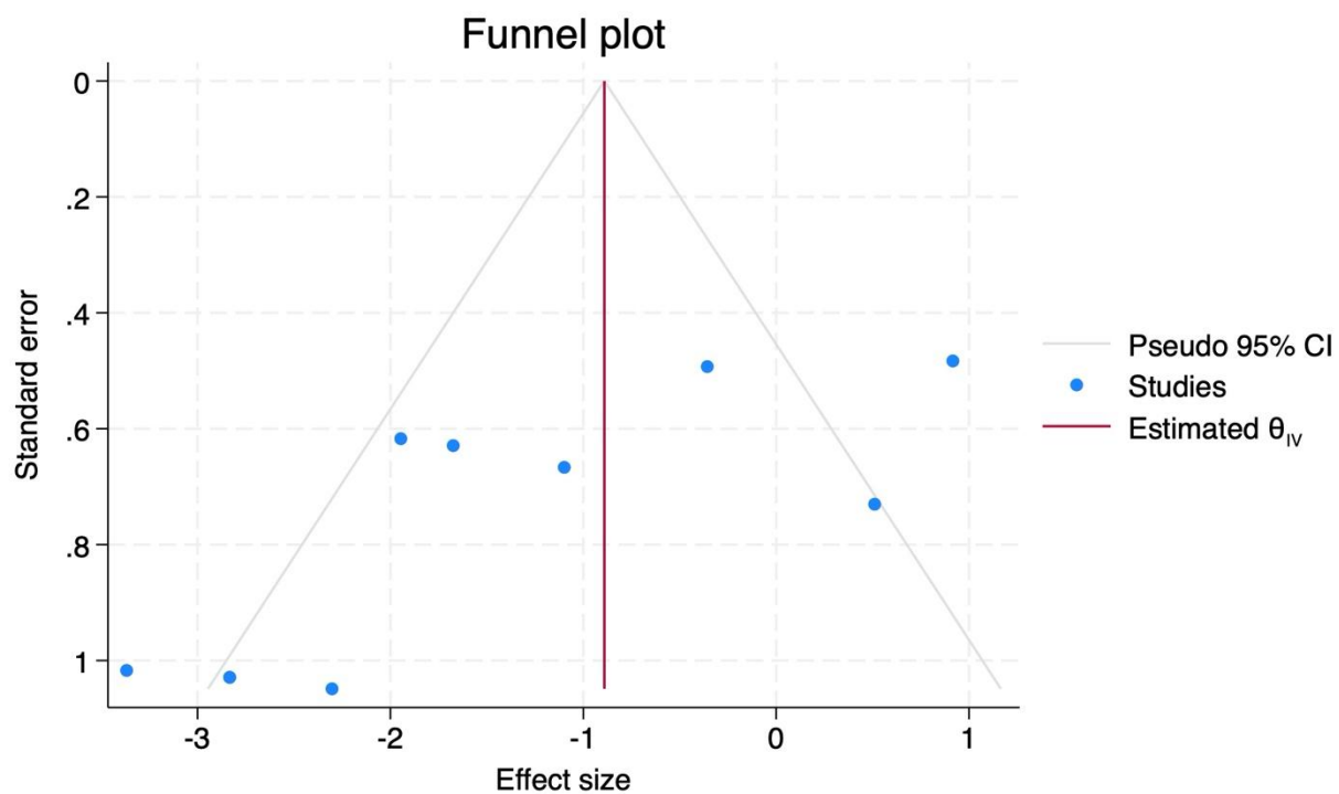
Supplementary Figure 3 Funnel plot for pathologic complete response.
