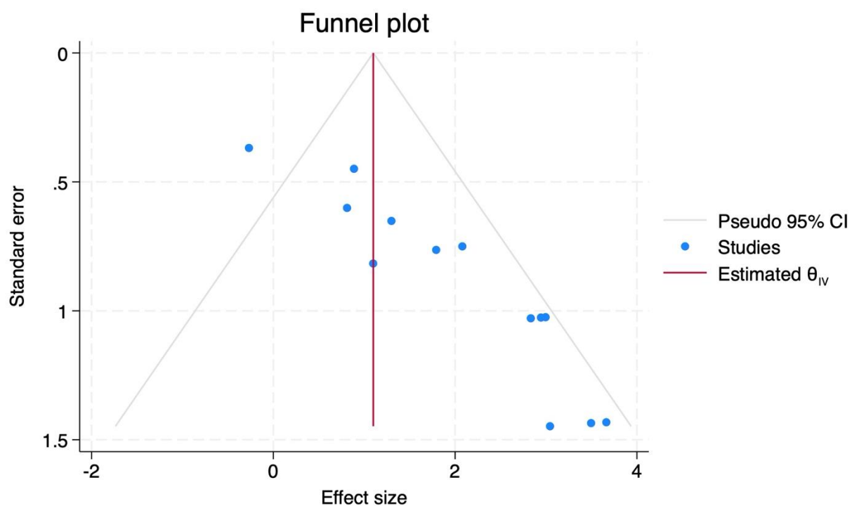
Supplementary Figure 4 Funnel plot for resection rate.
