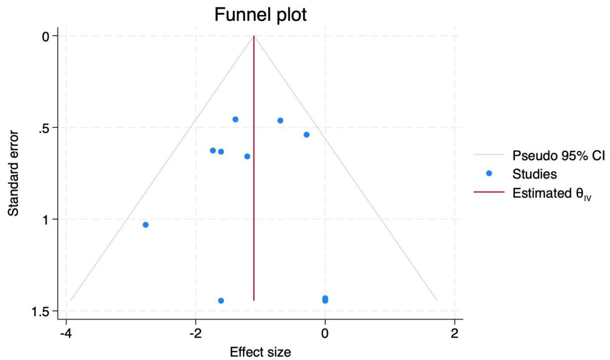
Supplementary Figure 5 Funnel plot for grade 3–4 treatment-related adverse events.
