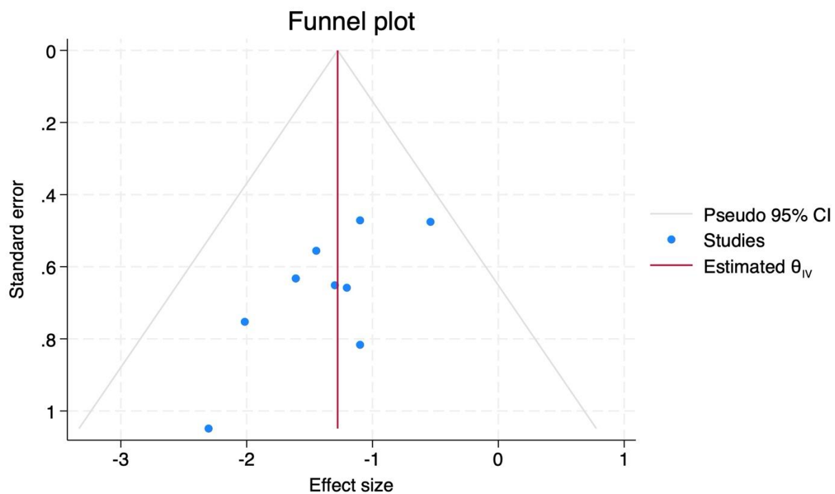
Supplementary Figure 1 Funnel plot for major pathologic response.
