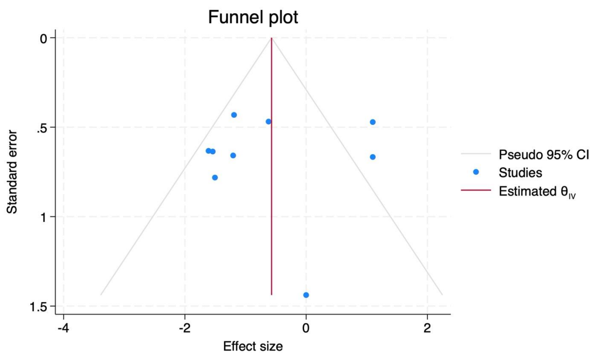
Supplementary Figure 2 Funnel plot for overall response rate.
