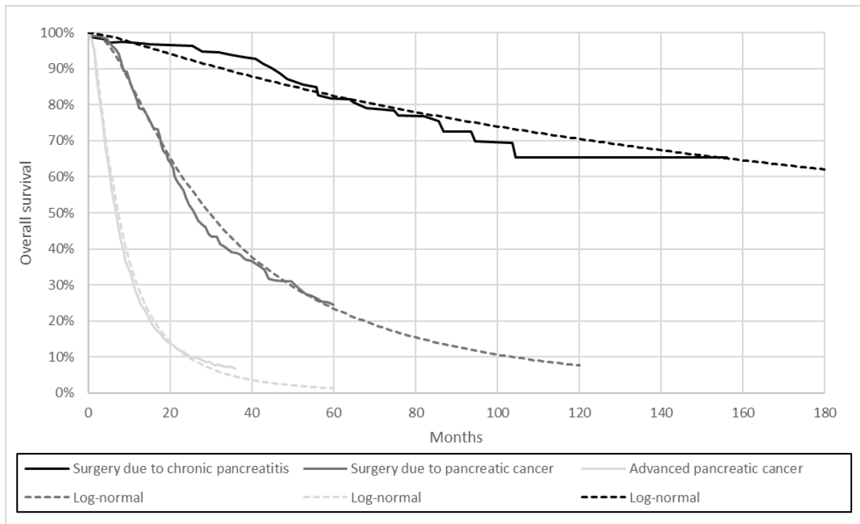
Supplementary Figure 1 Overall survival parametric extrapolation.
