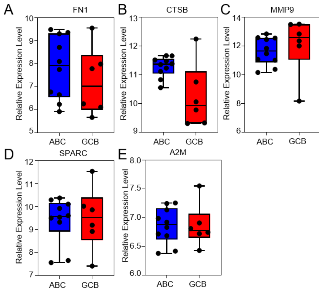
Figure S1. The subtypes analysis in GSE109027. A-E: The FN1, CTSSB, MMP9, SPARC and A2M expression in GCB and ABC-like DLBCL patients. GCB: germinal center B; ABC: activated B-like; DLBCL: Diffuse large B-cell lymphoma.
