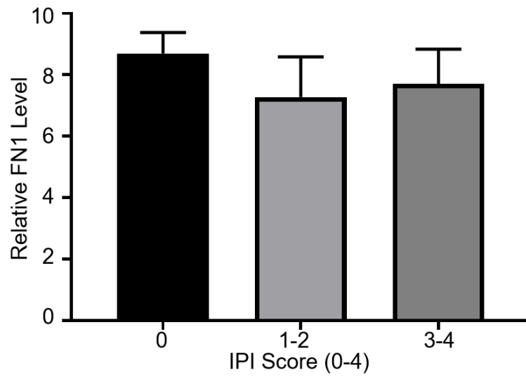
Figure S2. The correlation analysis between FN1 and IPI score in GSE109027. IPI: International prognostic index.
