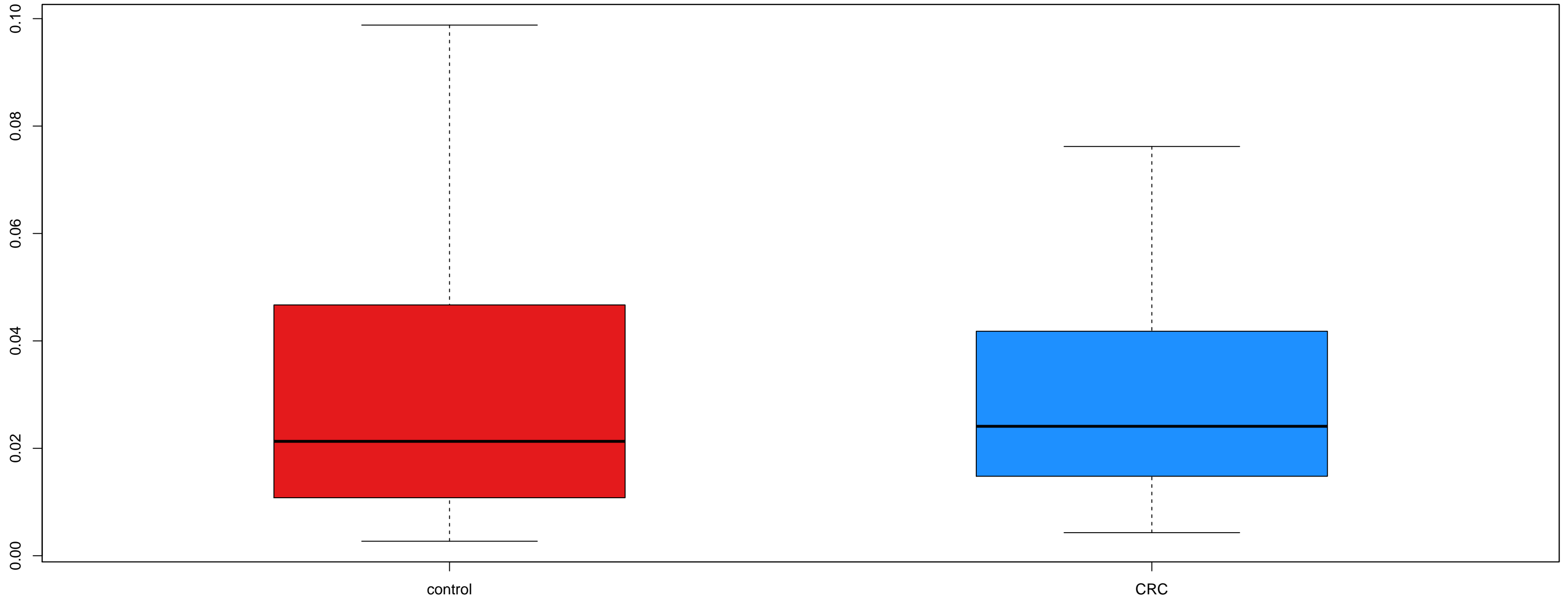
Simpson(p=0.503)
