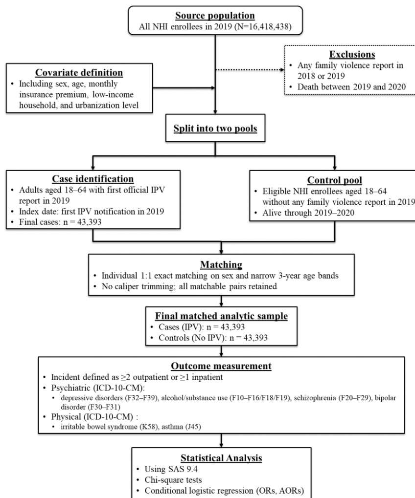
Figure S1. Cohort assembly and analysis flow
