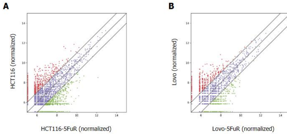
Supplementary Figure 1 The scatter plot figuratively expressed the changes of circRNA expression between the HCT116-5FuR cells and HCT116 cells and Lovo-5FuR cells and Lovo cells. A: HCT116-5FuR cells and HCT116 cells; B: Lovo-5FuR cells and Lovo cells.
