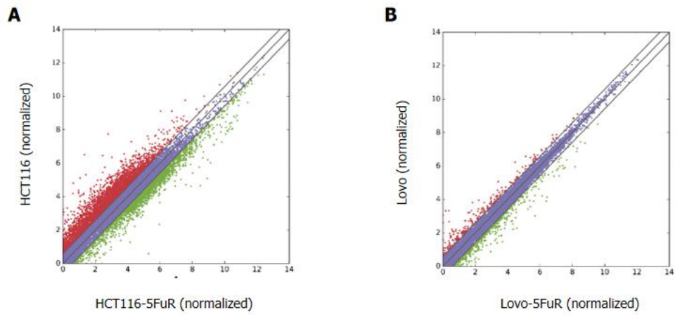
Supplementary Figure 2 The scatter plot figuratively expressed the changes of mRNA expression between the HCT116-5FuR cells and HCT116 cells and Lovo-5FuR cells and Lovo cells. A: HCT116-5FuR cells and HCT116 cells; B: Lovo-5FuR cells and Lovo cells.
