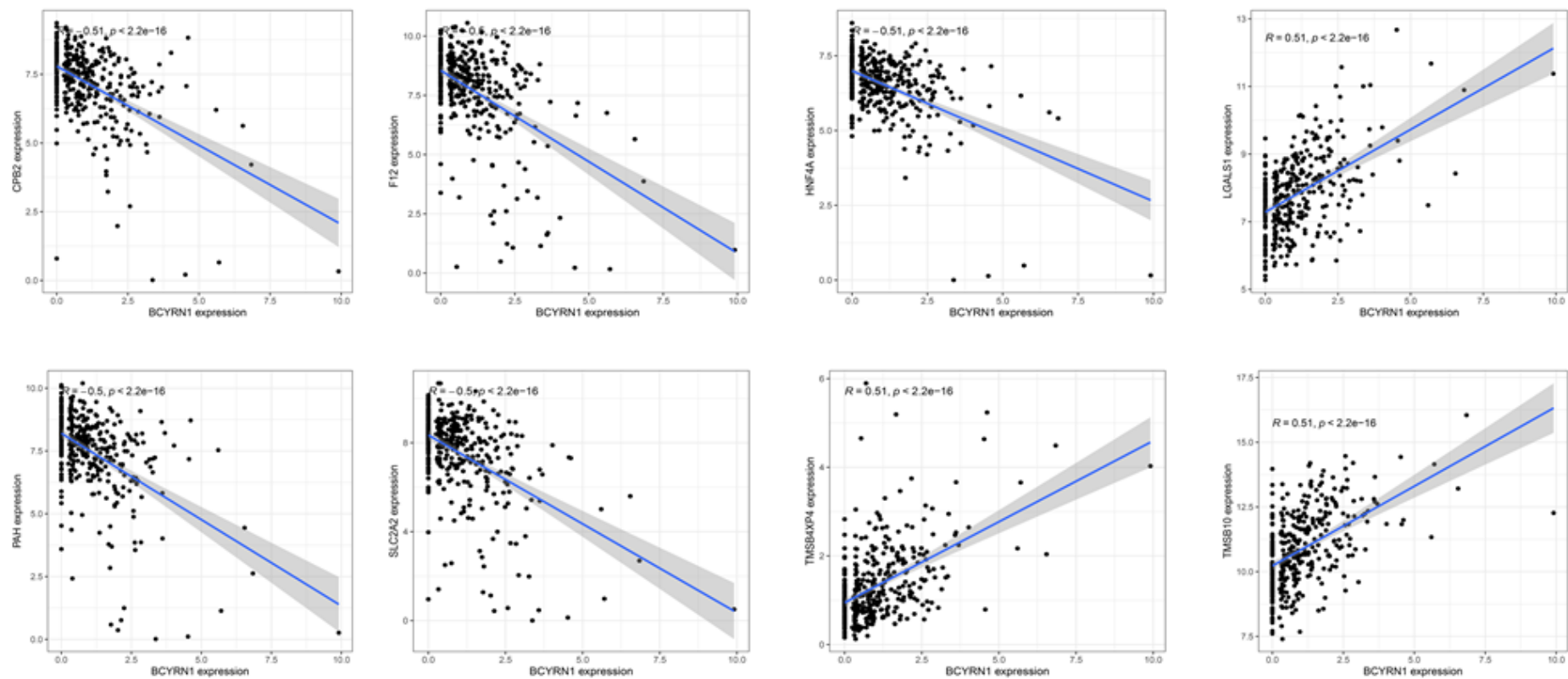
Supplementary Figure 1 Scatter plot of co-expression correlation of 8 genes that met the screening criteria.
