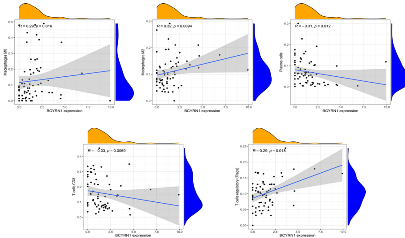
Supplementary Figure 2 Scatter plot of the correlation between the expression of brain cytoplasmic RNA1 and the levels of five selected immune cell infiltrates.
