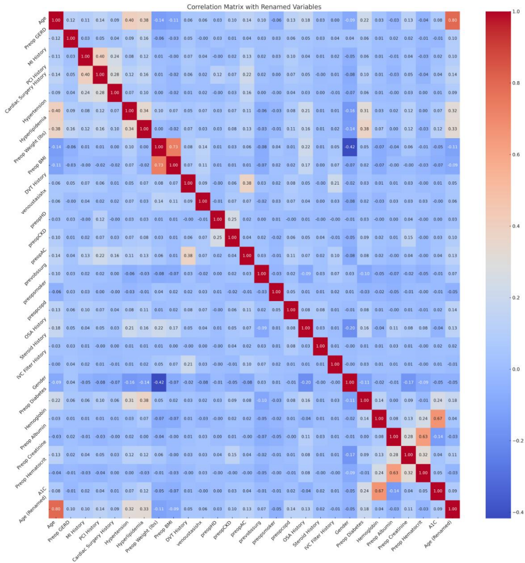
Supplementary Figure 1 Correlation matrix with renamed variables.
