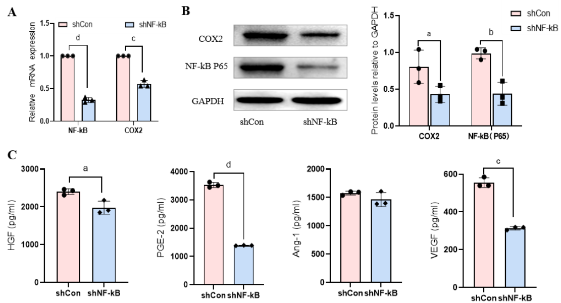
Supplementary Figure 3 Knockdown of NF- \kappa B significantly inhibited the expression of COX2 and the secretion of cytokines.
