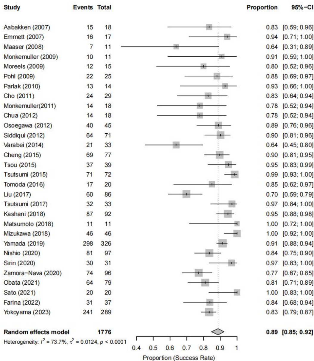
Supplementary Figure 2 Forest plot for enteroscopy success.
