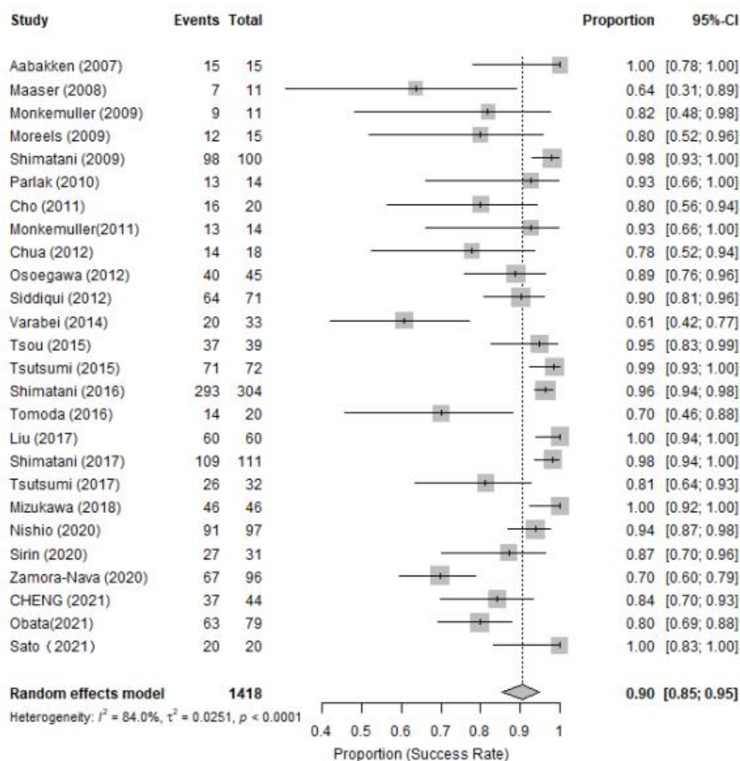
Supplementary Figure 3 Forest plot for diagnostic success.
