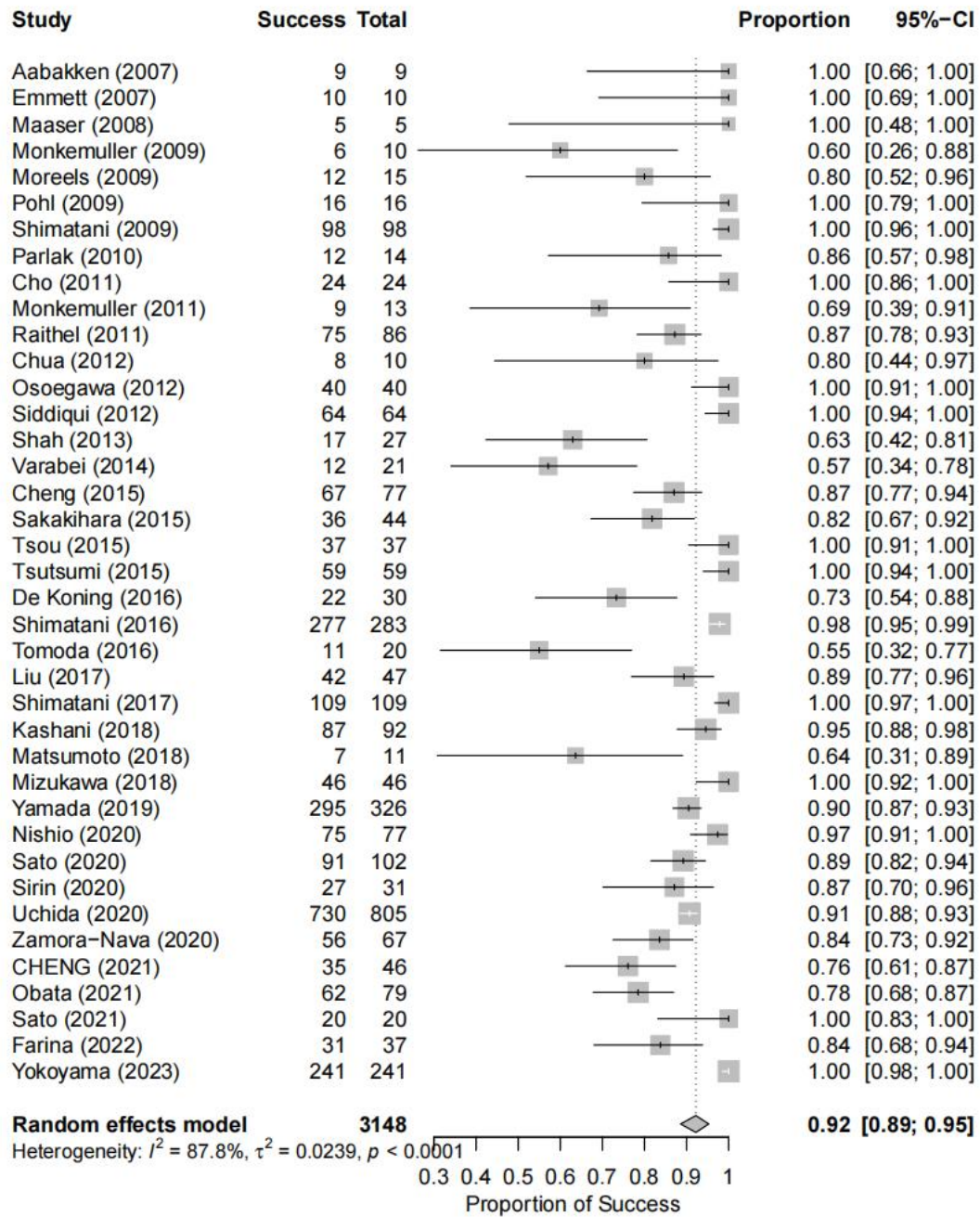
Supplementary Figure 4 Forest plot for procedural success.
