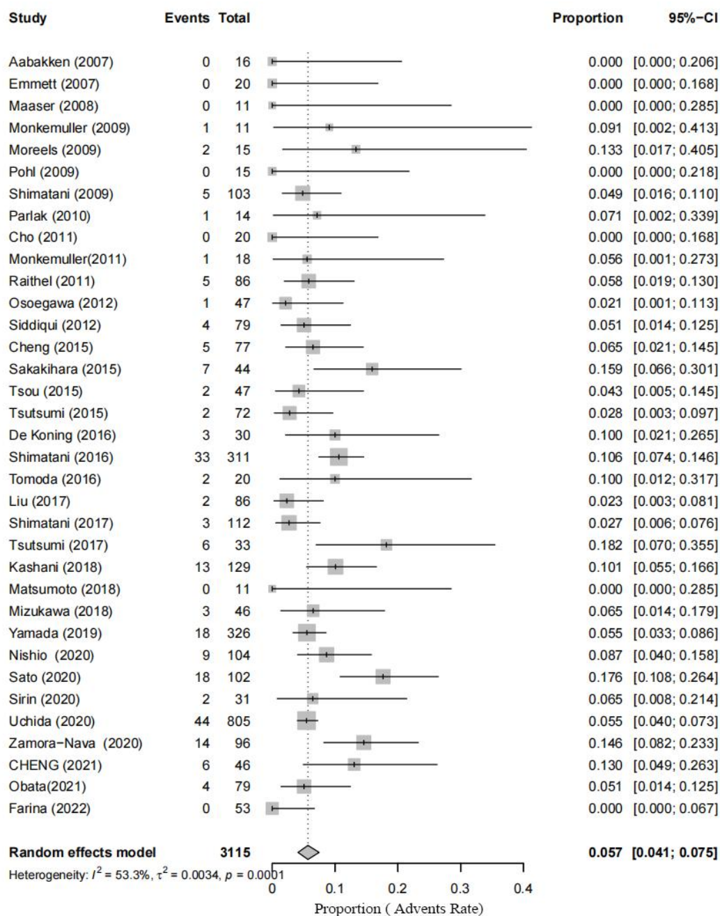
Supplementary Figure 5 Forest plot for adverse events.
