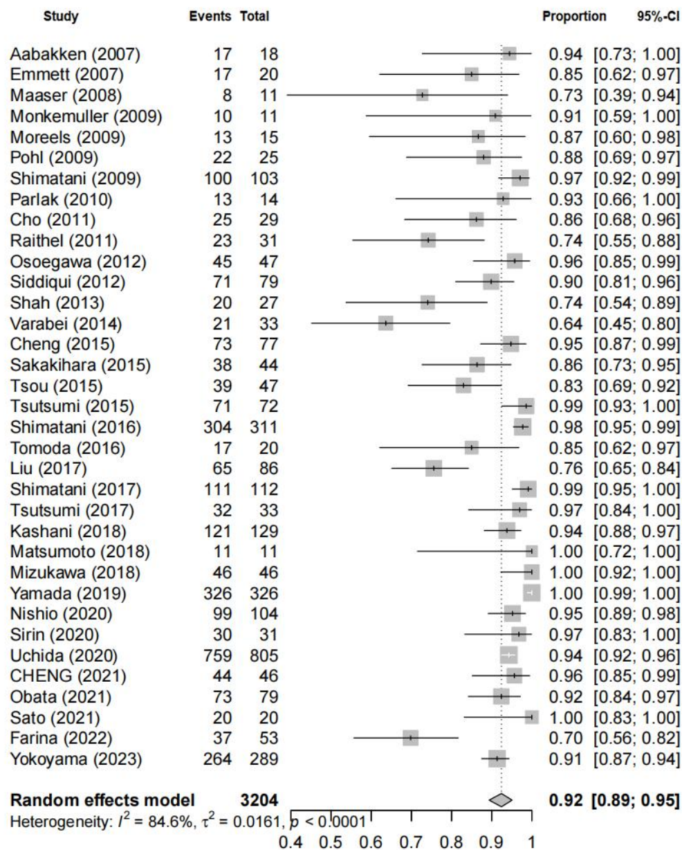
Supplementary Figure 1 Forest plot for papilla reached.
