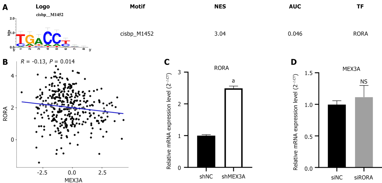
Figure 7 RORA can be regarded as a downstream gene for MEX3A. A: Analysis of transcription factors found a binding motif for the transcription factor RORA at the promoter of the differential genes associated with MEX3A expression; B: Correlation between RORA and MEX3A; C and D: QPCR was used to detect mRNA level of RORA and MEX3A after knockdown of MEX3A and RORA. Data are presented as the mean \pm SD. a P < 0.001 .
