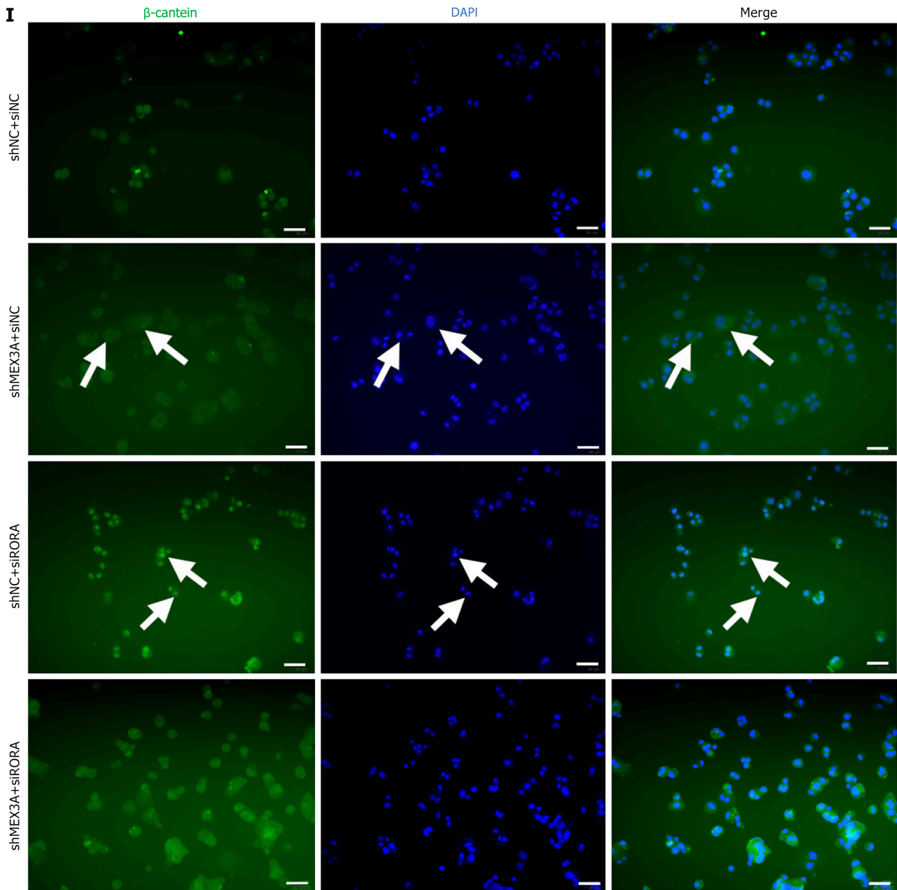
Figure 8 Role of RORA in hepatocellular carcinoma as a downstream gene for MEX3A. A-C: Real-time fluorescent quantitative PCR and western blotting detection of the knockdown efficiency of MEX3A and RORA; D: Cell counting kit-8 assay detection of the proliferative ability of the cells divided into four groups of HepG2 cells ("c" represents significant difference between the shNC + siNC and shMEX3A + siNC groups; "d" represents significant difference between the shMEX3A + siRORA and shMEX3A + siNC groups); E and F: Crystal violet staining was used to detect the clone formation ability of the cells divided into four groups; G and H: Western blotting detection of the effect of MEX3A or RORA silencing on expression of proteins in the Wnt/ \beta -catenin pathway. Data are presented as the mean \pm SD; I: Immunofluorescence was used to detect the accumulation of \beta -catenin in the nucleus. a P < 0.05 , b P < 0.01 , c P < 0.001 , d P < 0.001 . Scale bar = 50 \mu m.
