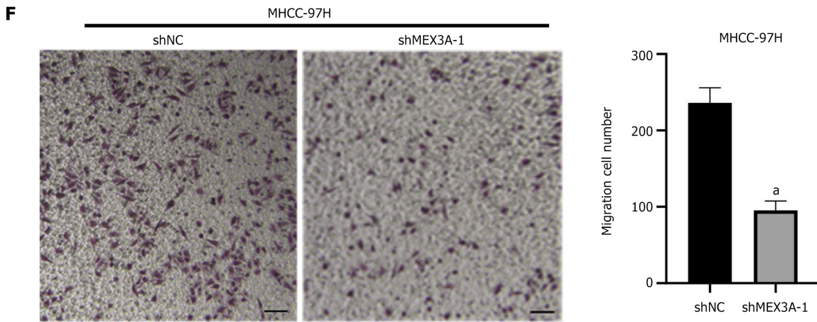
Figure 6 Effect of MEX3A on cell migration in hepatocellular carcinoma. A: Gene set enrichment analysis (GSEA) of MEX3A expression and key pathways; red color represents statistically significant results. The size of the circle represents the number of genes; B: GSEA of MEX3A expression and epithelial-mesenchymal transition pathway; C and D: Cell scratch assay was used to detect the effect of MEX3A on cell migration; E and F: Transwell assay was used to detect the effect of MEX3A on hepatocellular carcinoma migration. Data are presented as the mean \pm SD. a P < 0.01 , b P < 0.001 . Scale bar in C-F = 100 \mu m.
