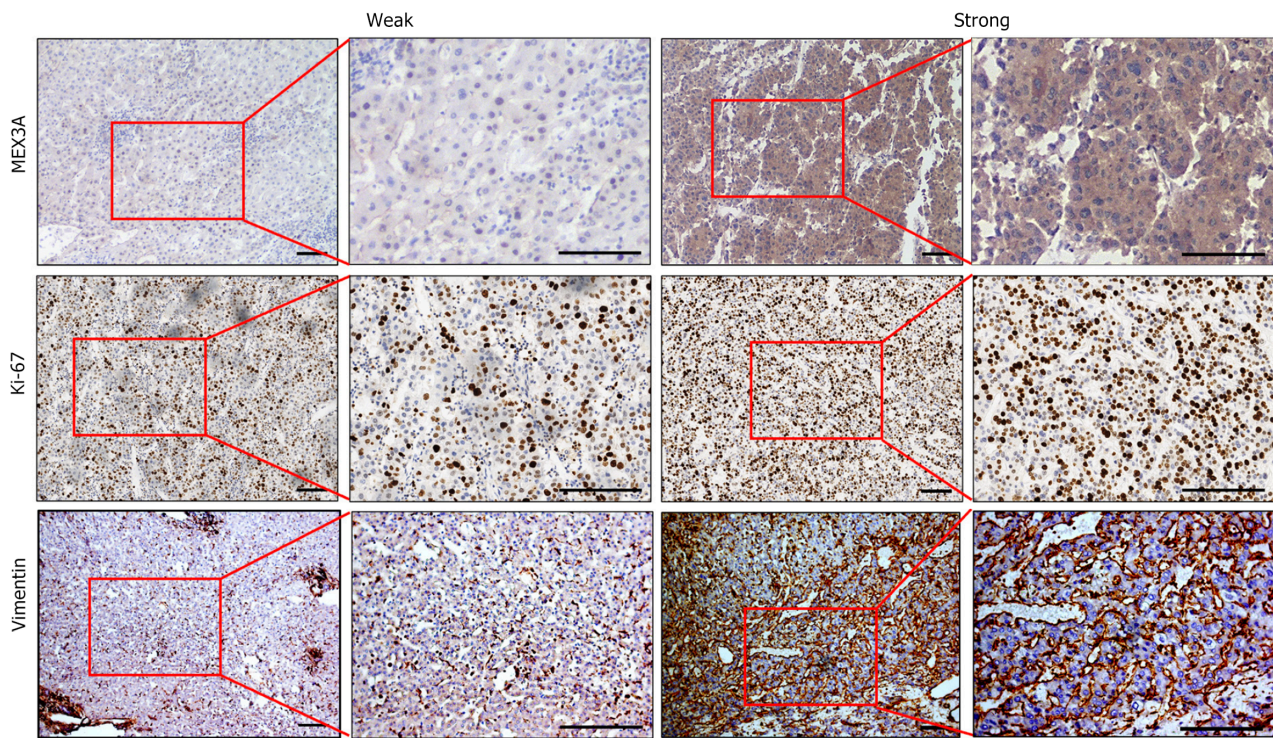
Figure 3 Low and high expression of MEX3A, Ki-67 and vimentin in hepatocellular carcinoma tissues. Scale bar = 100 and 50 \mu m.
