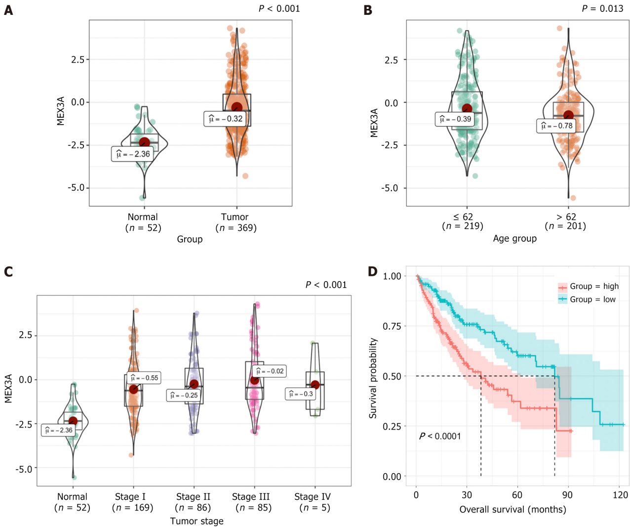
Figure 1 Analysis of MEX3A expression. A: Differential expression of MEX3A mRNA in hepatocellular carcinoma (HCC) and adjacent non-tumor tissues ( P < 0.001 ); B and C: Differential expression of MEX3A mRNA in HCC according to age ( P = 0.013 ) and tumor-node-metastasis stages ( P < 0.001 ); D: Kaplan-Meier survival analysis of MEX3A in HCC ( P < 0.0001 ).
