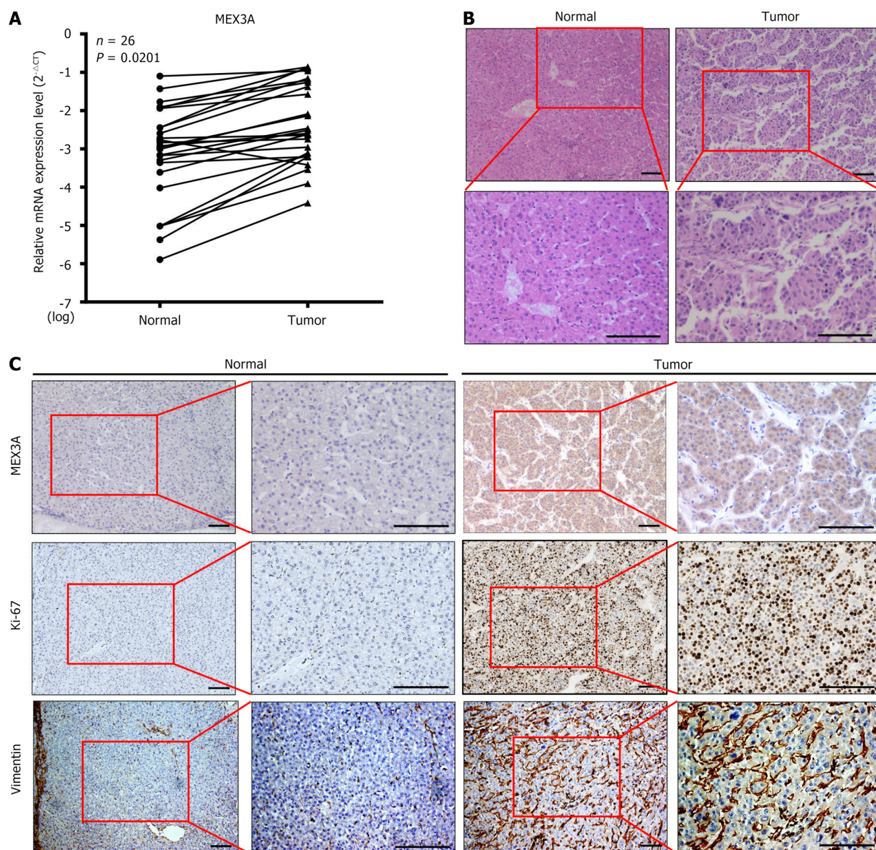
Figure 2 MEX3A expression in clinical specimens. A: Real-time fluorescent quantitative PCR was used to detect expression of MEX3A mRNA in hepatocellular carcinoma (HCC) and adjacent tissues; B: Hematoxylin and eosin staining in HCC and adjacent tissues; C: Expression of MEX3A, Ki-67 and vimentin in HCC and adjacent tissues was detected by immunohistochemistry. Scale bar = 100 and 50 \mu m.
