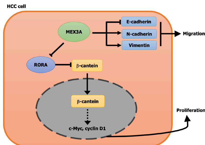
Figure 9 Schematic representation of mechanisms by which MEX3A promotes hepatocellular carcinoma cell proliferation and migration. HCC: Hepatocellular carcinoma.
