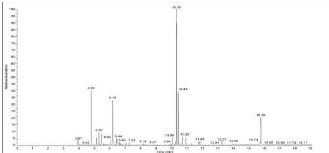
Figure 2 QC total ion current diagram.
