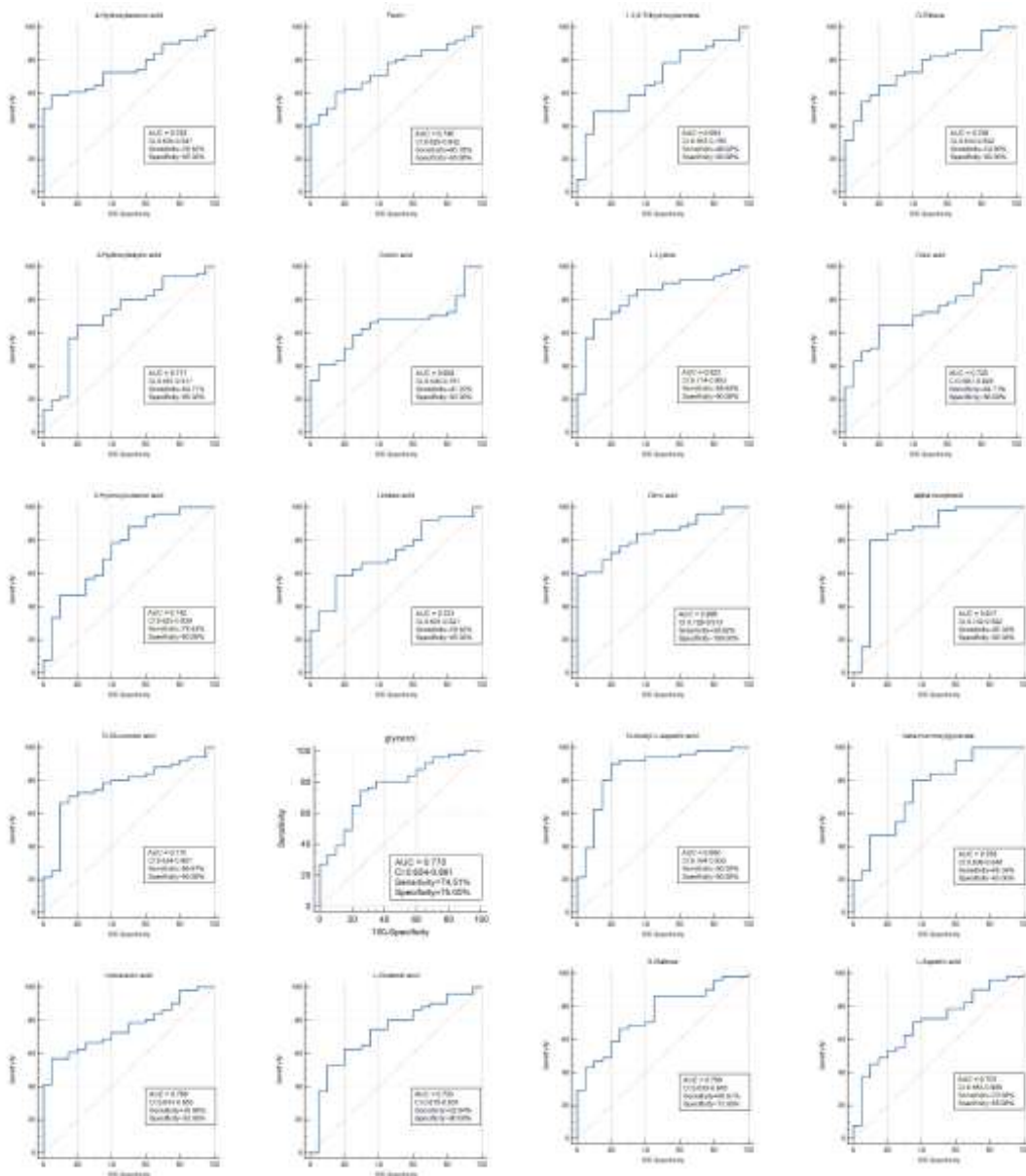
Figure 3 Differential metabolite ROC curve
